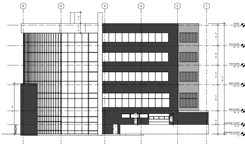
① WEST ELEVATION 1/8" = 1'-0"
