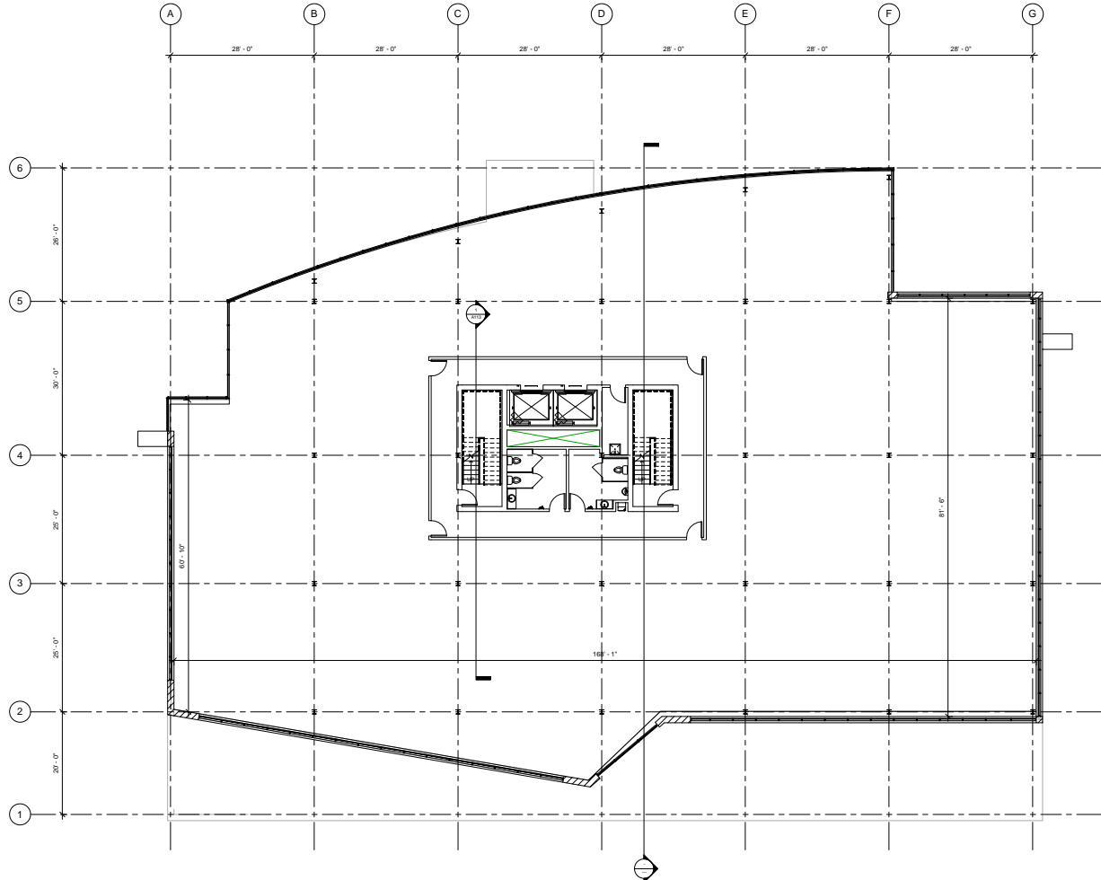
① 3RD FLOOR 1/8" = 1'-0"
